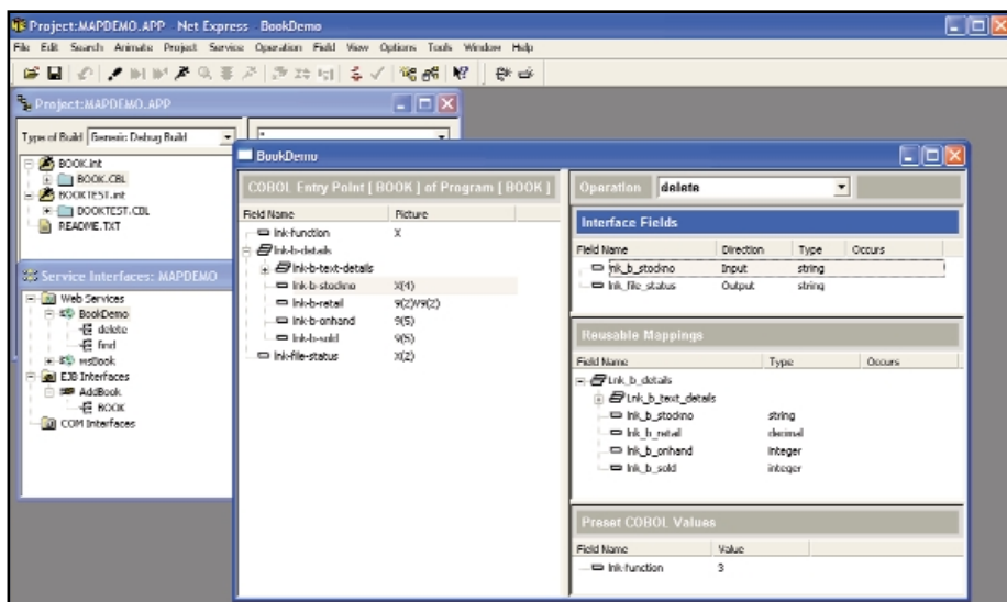
The Interface Mapping Toolkit functionality within Net Express enables programmers to expose an existing COBOL program interface as a Web service, EJB or COM component with a simple point-and-click interface.
